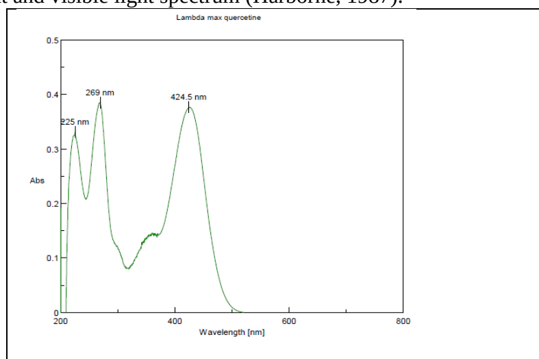
Figure 1. Maximum Wavelength
